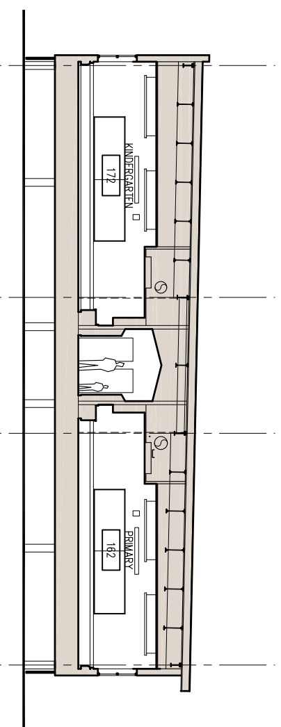
BUILDING SECTION THROUGH CLASSROOMS
